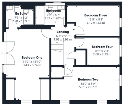
Floor 1 Building 1
