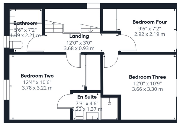
Floor 1 Building 1
