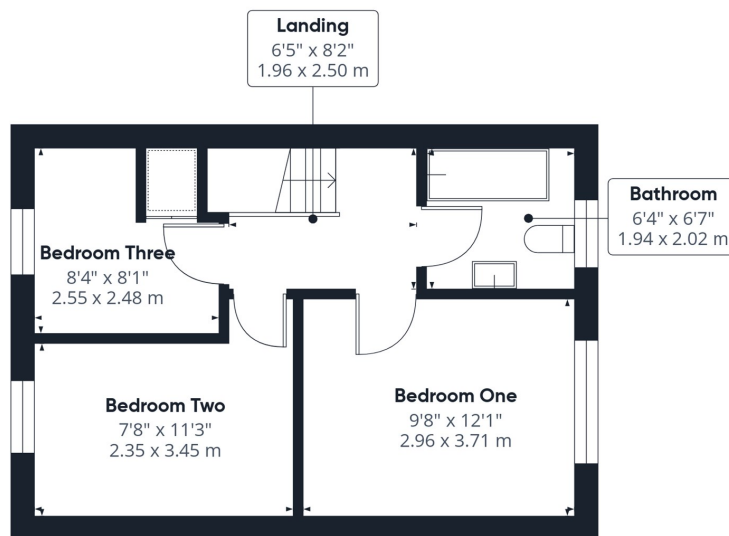
Floor 1
